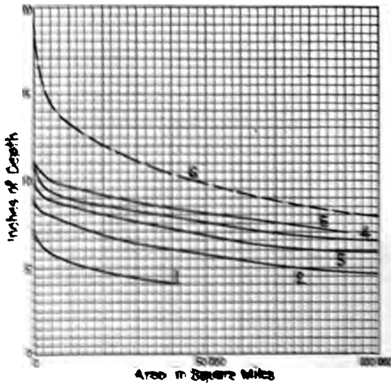
FIG. 10. Area-depth rainfall relations Ohio storm of March 25-27, 1913.
